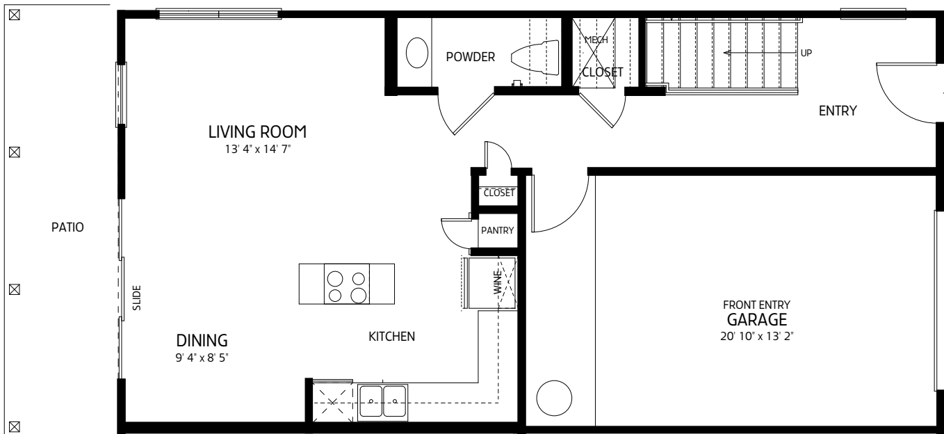
FIRST FLOOR 588 S.F.
